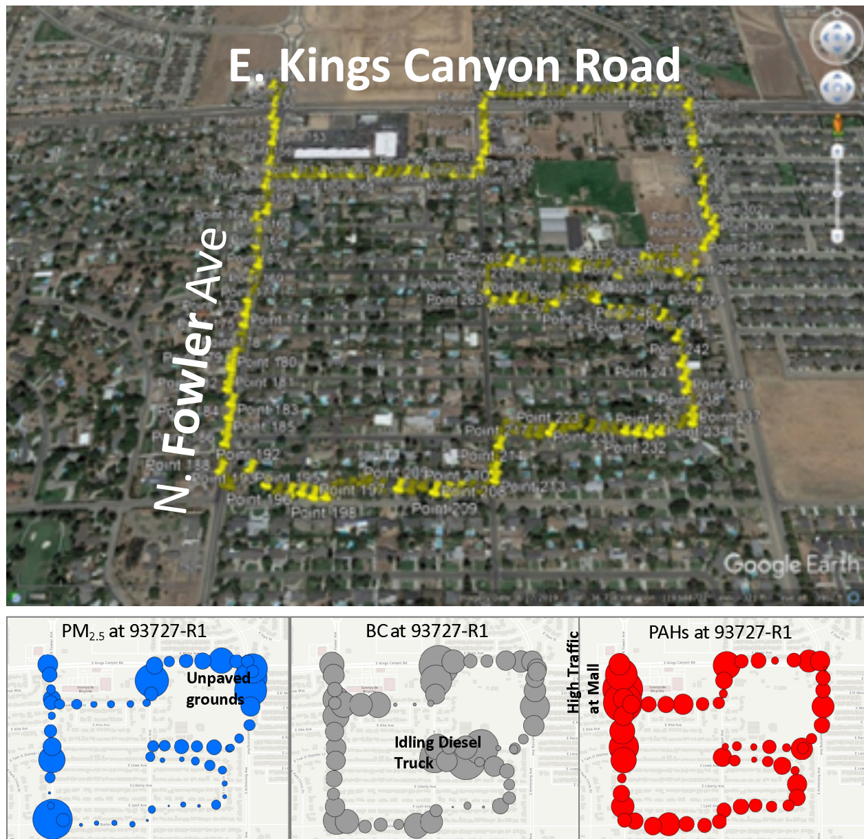
Figure 16. PM 2.5 , BC, and PAHs Concentrations and GPS Waypoints Measured at 93727-R1 on a Sampling Period.
