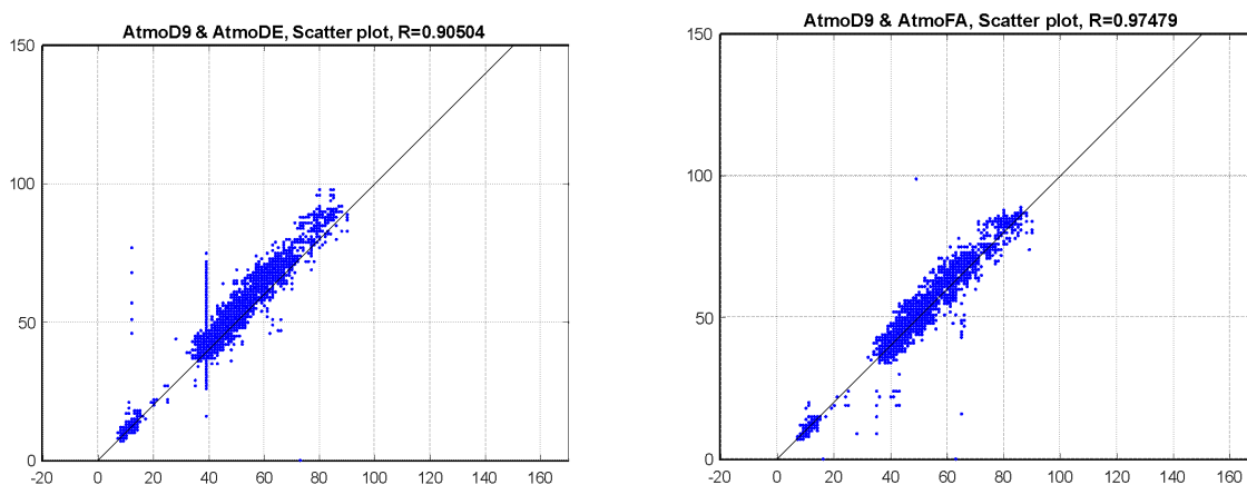
Figure 26. Inter-sensor analysis of Atmotube Pro PM2.5. Scatter plots of Atmotube Pro D9 vs. Atmotube Pro DE (Left). Atmotube Pro D9 vs. Atmotube Pro FA (Right).
