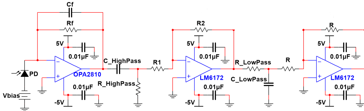
Figure 4. Photodiode Receiver Circuit
