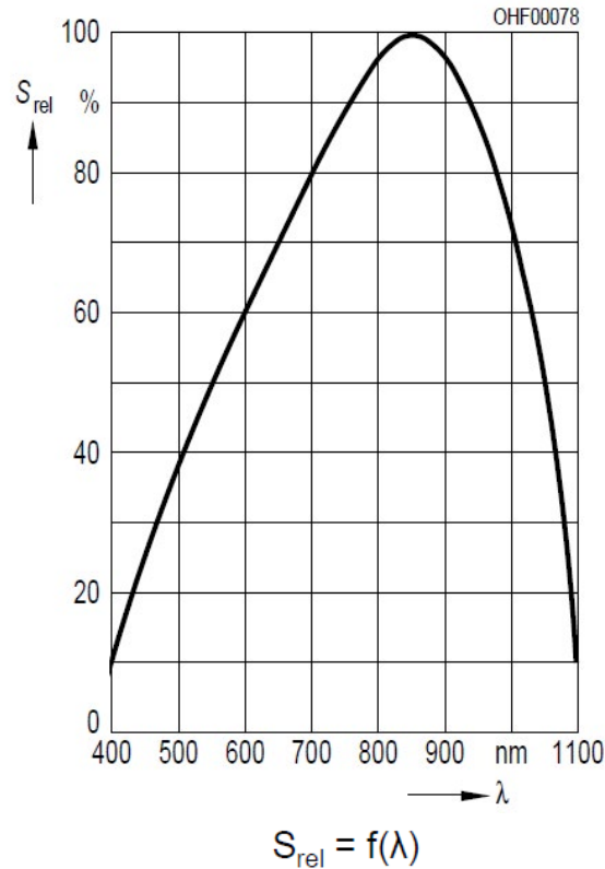
Figure 5. BPX61 Photodiode Relative Spectral Sensitivity as a Function of Wavelength
